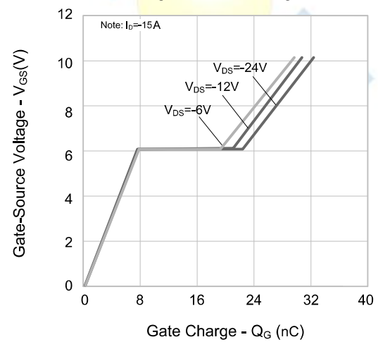
Figure 6. Gate Charge
