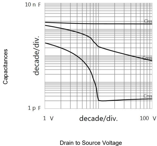
Figure 5. Capacitances
