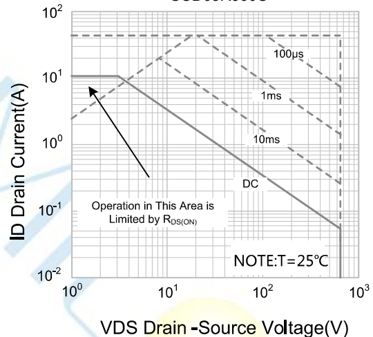
Figure 9-2. Max. Safe Operating Area of SCD65R380C
